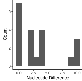
IGHV3-I3JG*01 20 sequences assigned 7 (35%) exact matches, in which: 7 unique CDR3 3 unique J
