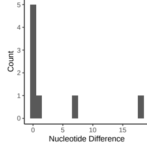
IGHV3-37F2*02 8 sequences assigned 5 (62.5%) exact matches, in which: 5 unique CDR3 3 unique J
